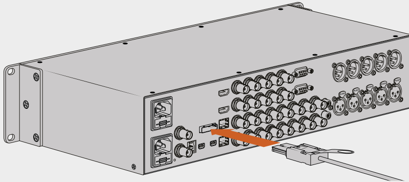
UltraStudio 4K Extreme features a PCIe port for connection to an external PCIe adapter card that is installed in your computer
