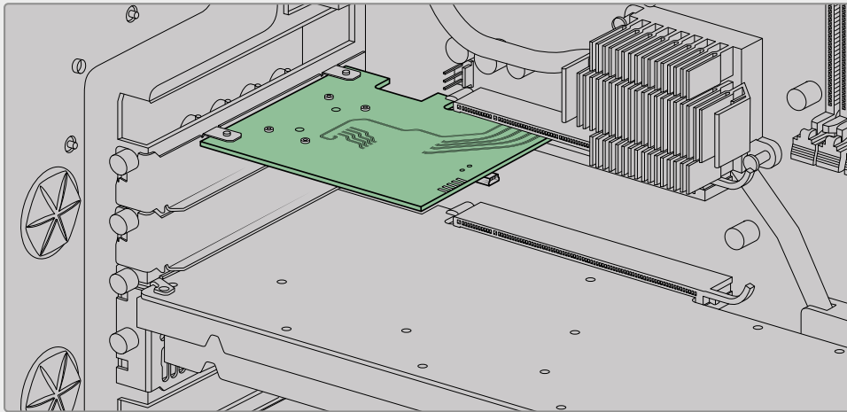
The PCIe adapter card is inserted into a PCIe Gen 2 slot inside your computer
